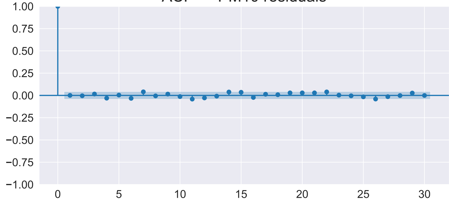
ACF — PM10 residuals
